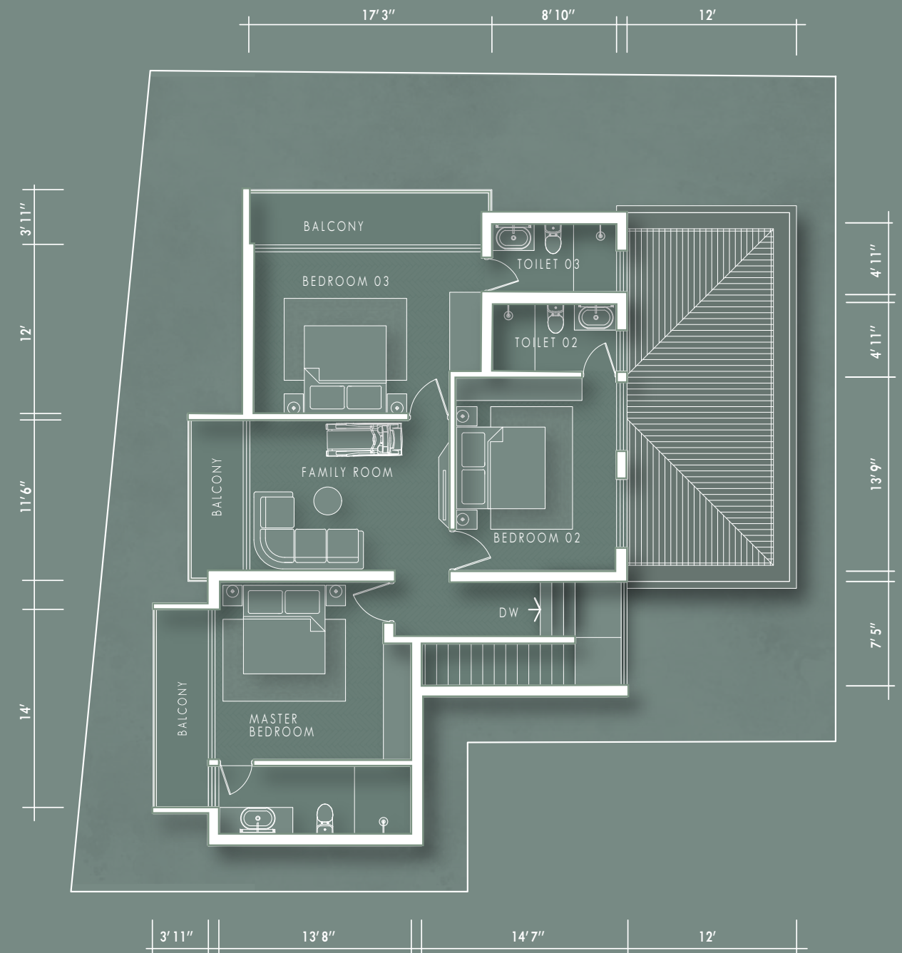
VILLA 03 First Floor 1250sqft
